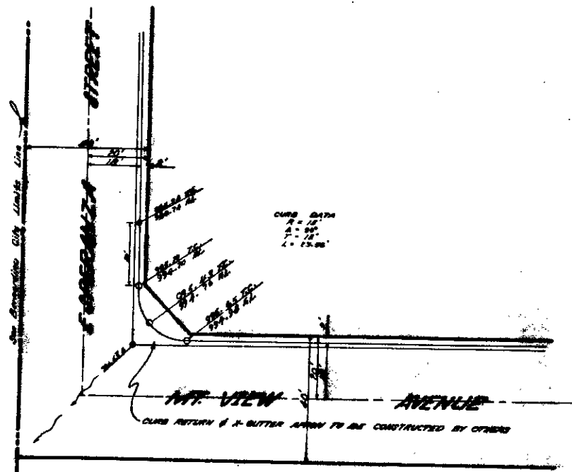
INTERSECTION DETAIL Scale: 1" = 20'
