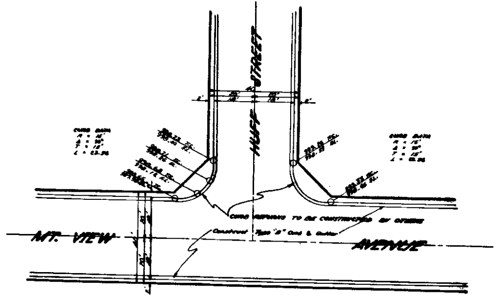
INTERSECTION DETAIL Scale: 1" = 20'
